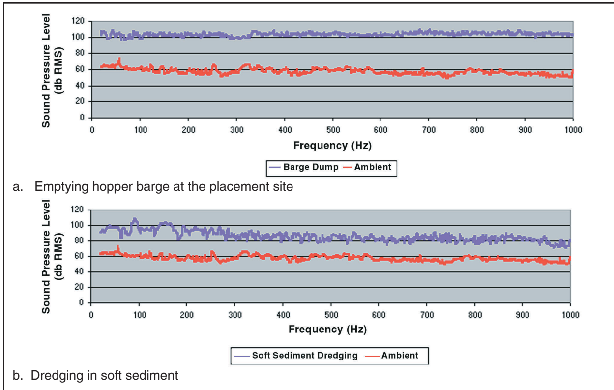
Figure 9. Sound pressure level produced when emptying hopper barge at the placement site and when dredging in soft sediment as measured over ambient conditions in Cook Inlet, Alaska
