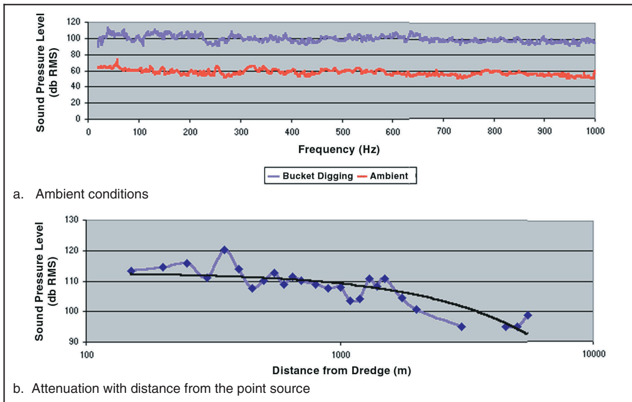
Figure 5. Sound pressure level produced by dredge bucket digging into coarse sediment as measured over ambient conditions and its attenuation with distance from the point source in Cook Inlet, Alaska
