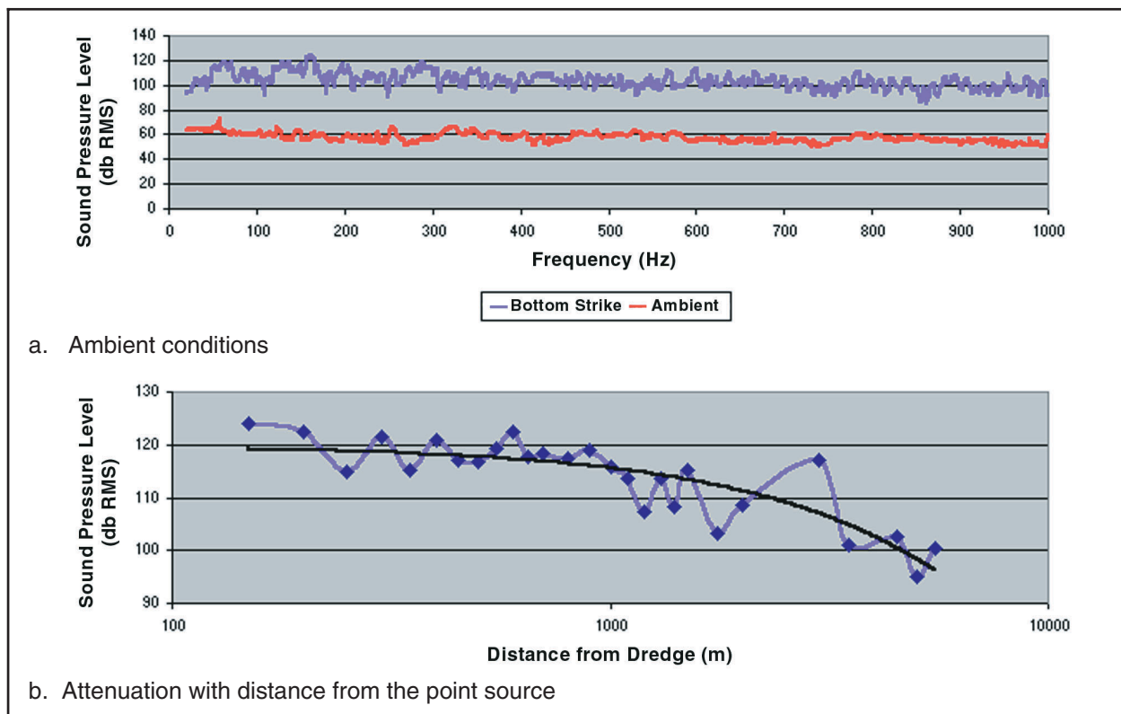
Figure 4. Sound pressure level produced by dredge bucket striking the channel bottom (coarse sediment and/or gravel) as measured over ambient conditions and its attenuation with distance from the point source in Cook Inlet, Alaska
