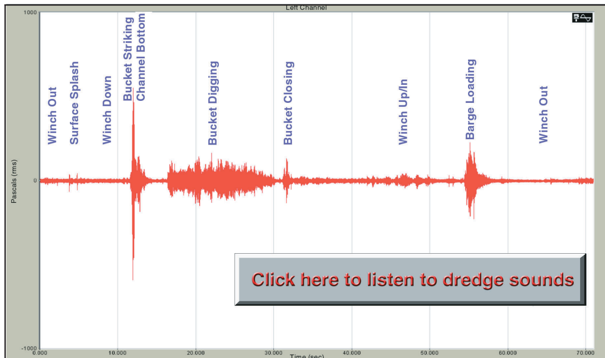
Figure 3. An example pressure waveform for a typical bucket deployment and retrieval cycle
