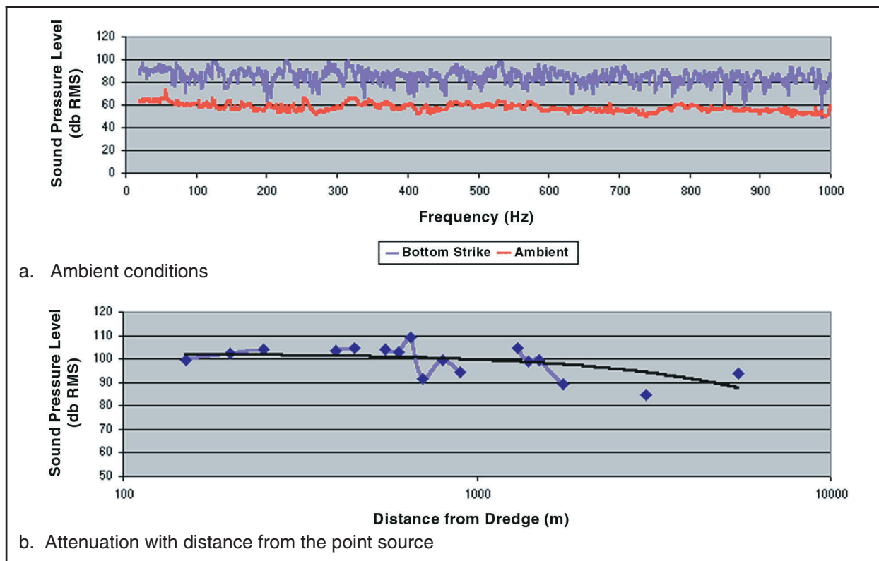
Figure 6. Sound pressure level produced by dredge bucket closing as measured over ambient conditions and its attenuation with distance from the point source in Cook Inlet, Alaska
