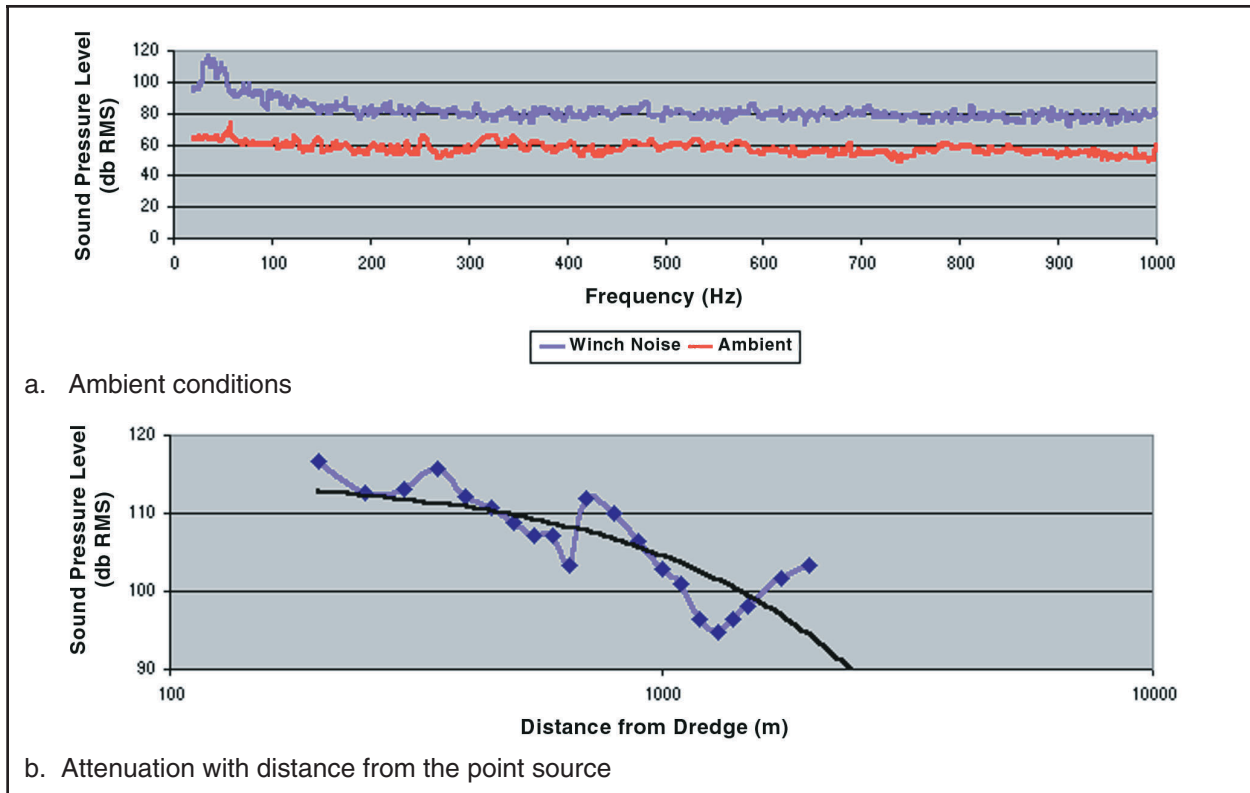
Figure 7. Sound pressure level produced from winch-generated noise measured over ambient conditions and its attenuation with distance from the point source in Cook Inlet, Alaska
