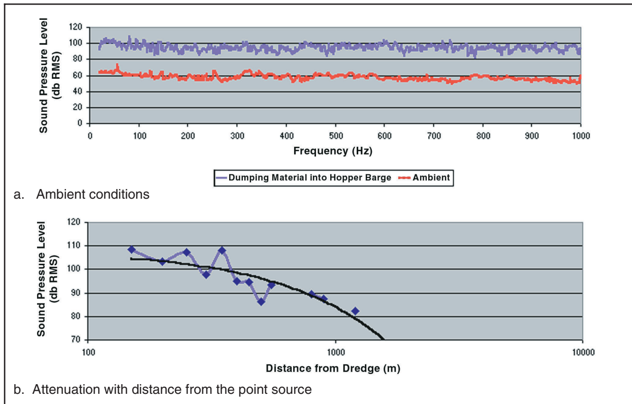
Figure 8. Sound pressure level produced from dumping material into hopper barge measured over ambient conditions and its attenuation with distance from the point source in Cook Inlet, Alaska
