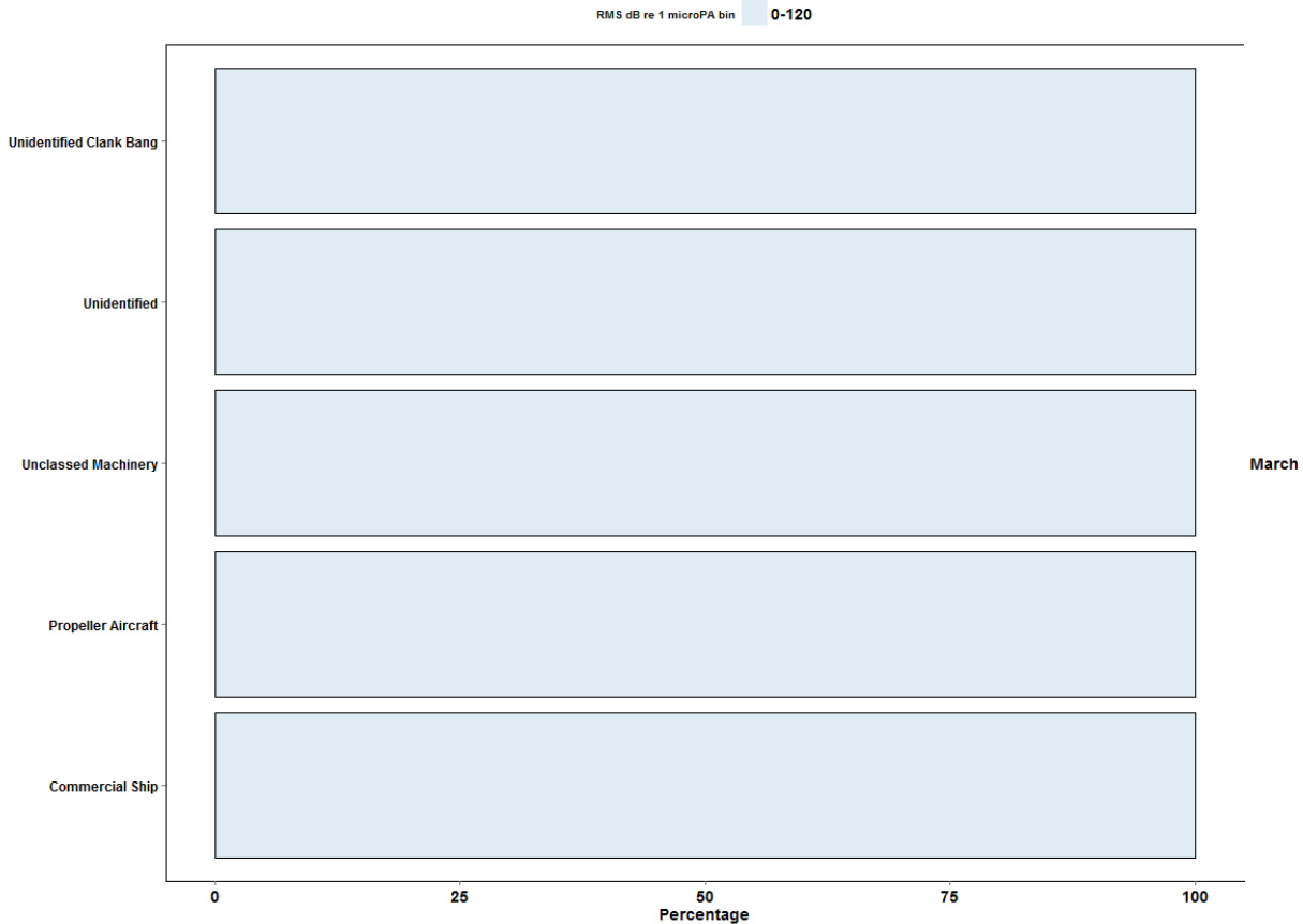
Figure 7: SPL distribution over time for each noise class detected in each location and month sampled in Cook Inlet Alaska, calculated as percentage of time over the total recording time for each month, within the bins 0-120, 120-125 and 125-153 dB. Bins are based on NOAA acoustic thresholds. Locations are A- Eagle River, B- Six Mile, C- Cairn Point, D- Fire Island, E- Trading Bay, F- Kenai River, and G- Tuxedni Bay.
