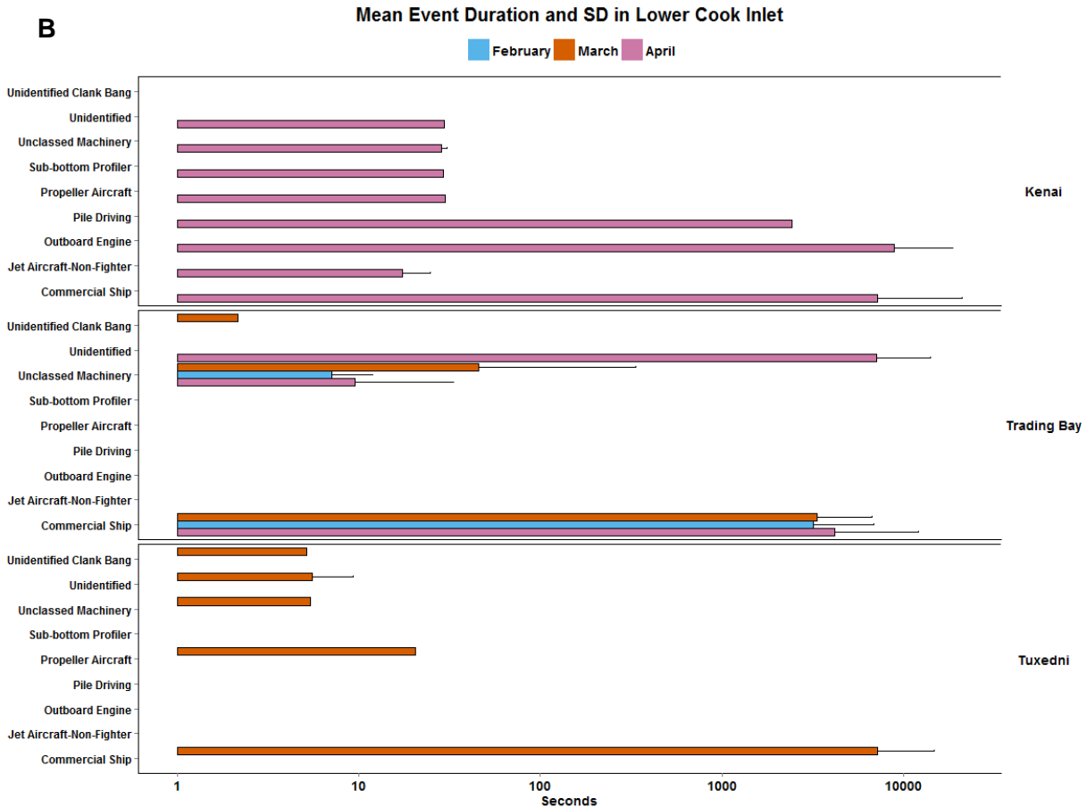
Figure 4: Average duration and standard deviation of noise classes detected at each site by month. Upper panel (A) includes the 4 locations sampled in the Upper Inlet (Cairn Point, Eagle River, Fire Island and Six Mile), and the lower panel (B) includes the 3 locations sampled in the Lower Inlet (Kenai, Trading Bay and Tuxedni). Note that up to three months were selected per location (see table 1), therefore, not all months were sampled in all locations.
