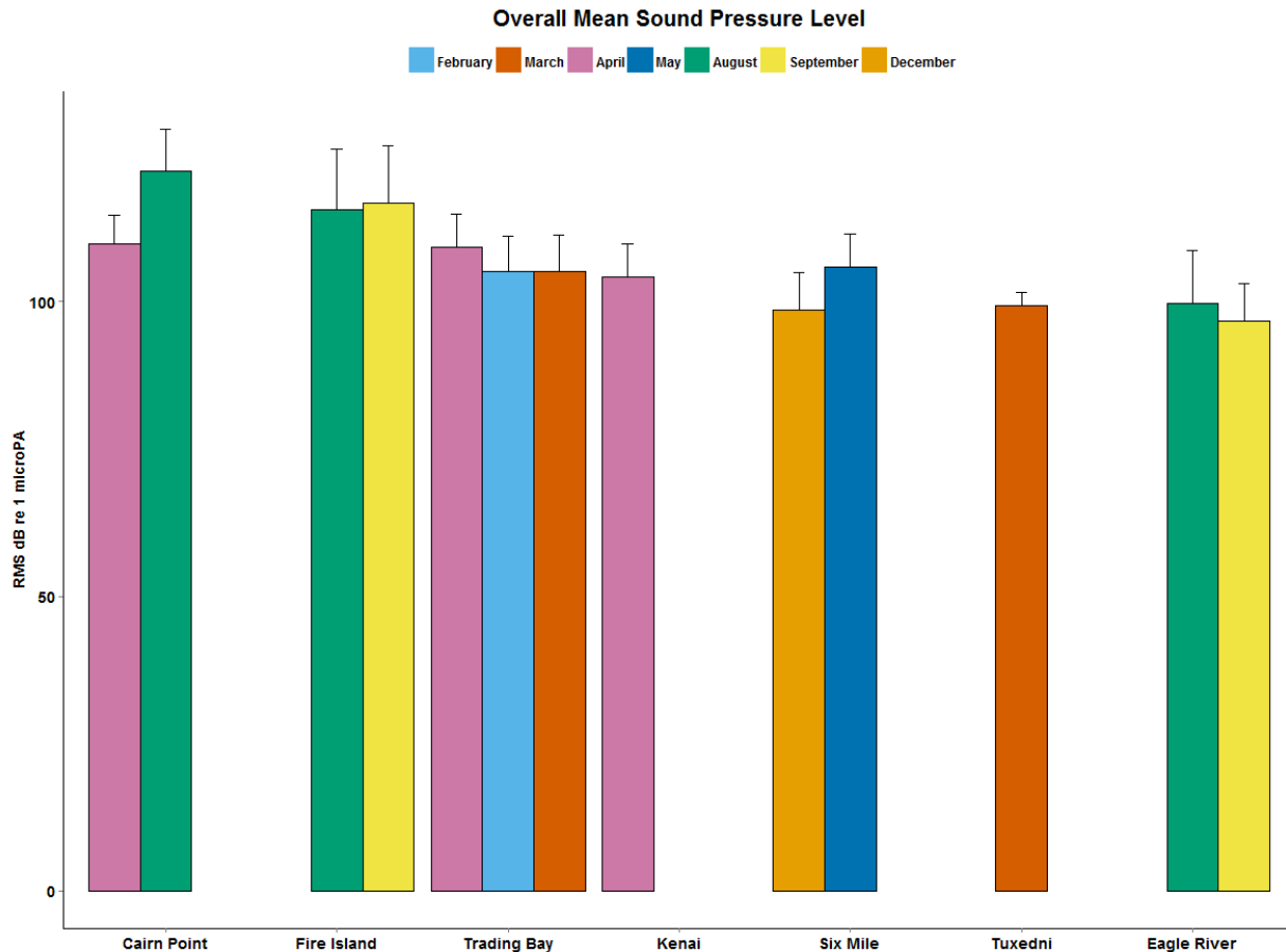
Figure 6: Overall mean anthropogenic sound pressure level (SPL) calculated as dB rms re 1 microPa and standard deviation from all the anthropogenic noise events of each location and month, independently of the noise class. Locations are ordered from noisiest to quietest.
