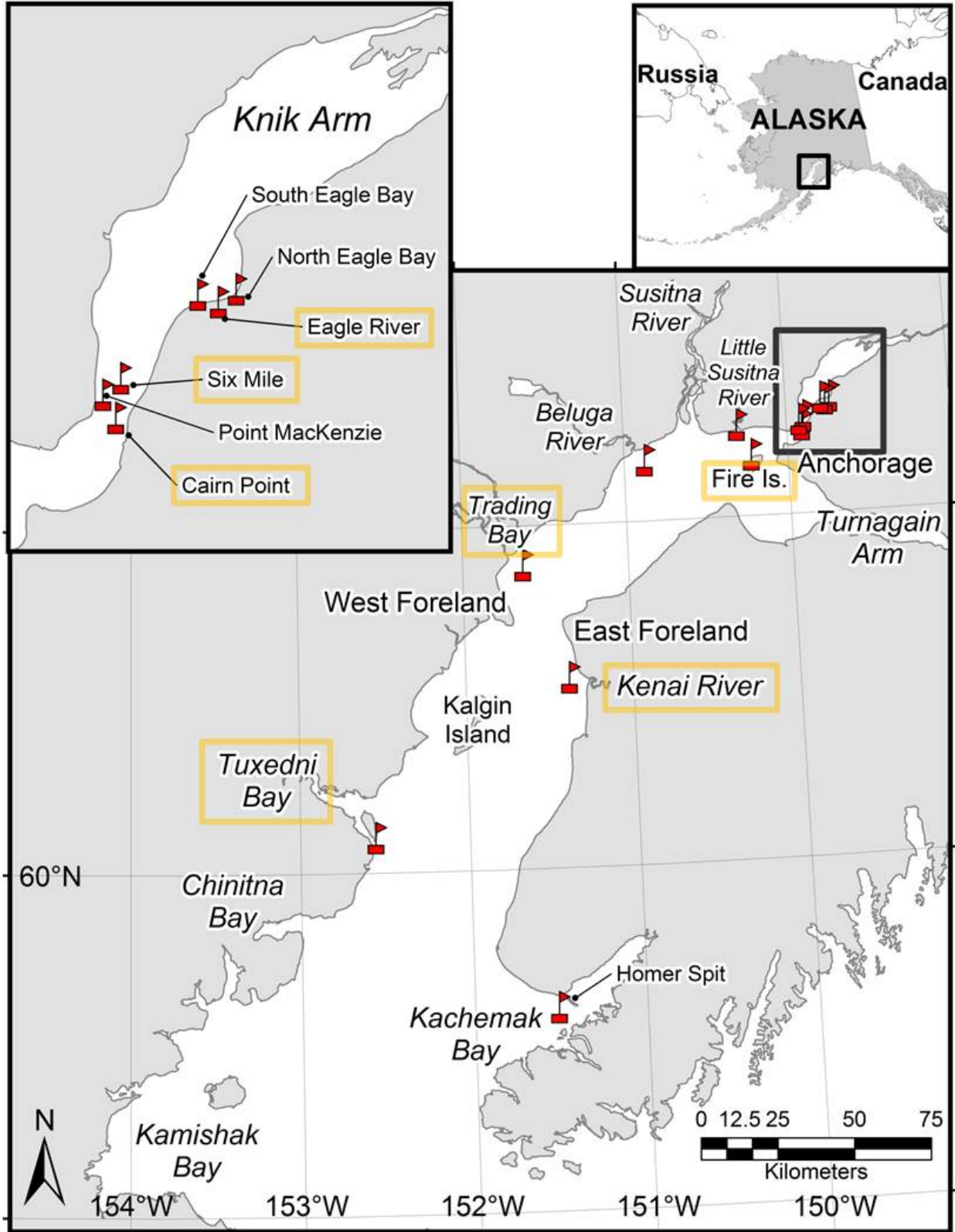
Figure 1: Acoustic mooring locations from CIBA research program in Cook Inlet, Alaska, deployed from July 2008 to May 2013. Data from mooring locations boxed in yellow were selected for this study.
