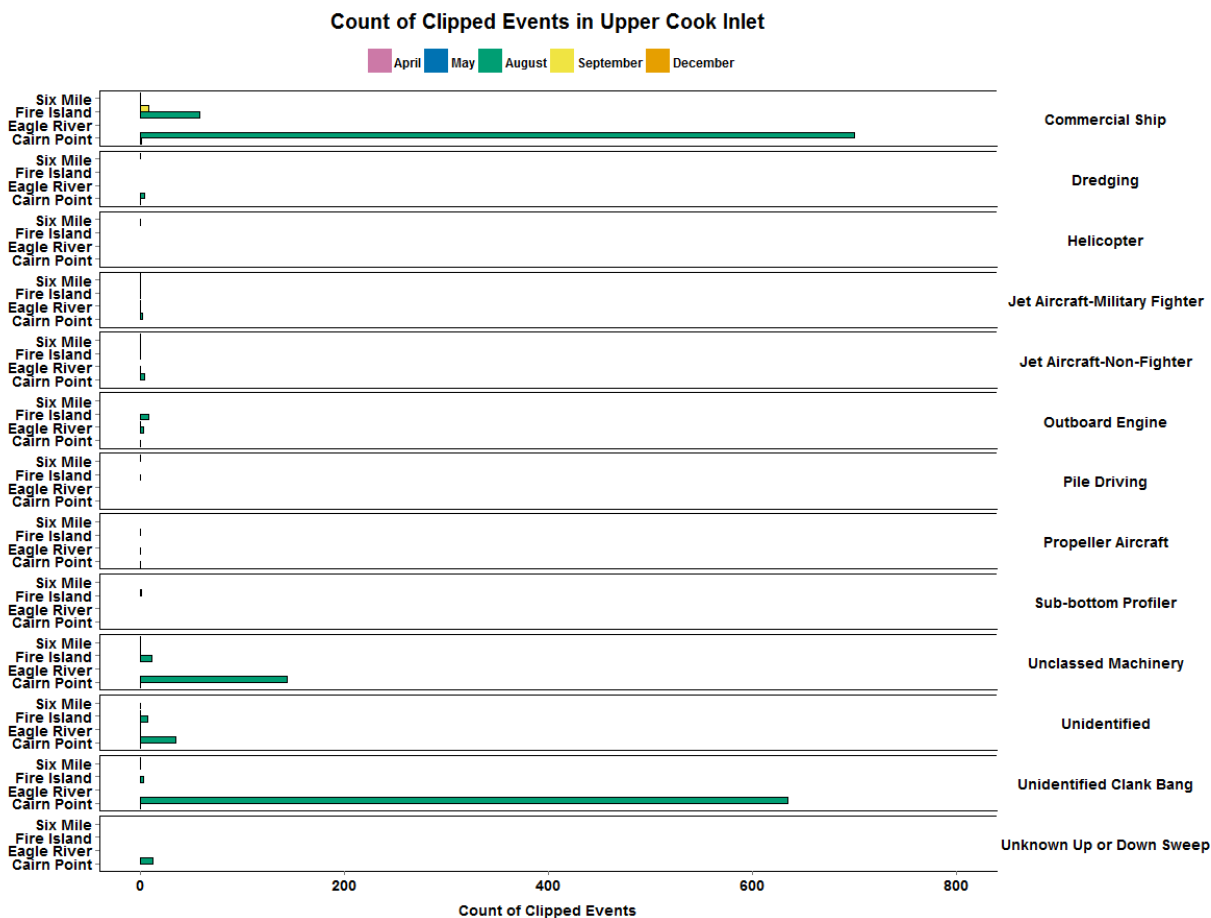
Figure 2: Number of clipped acoustic events by noise class, location and month for the 4 locations sampled in the upper Inlet (Cairn Point, Eagle River, Fire Island and Six Mile).
