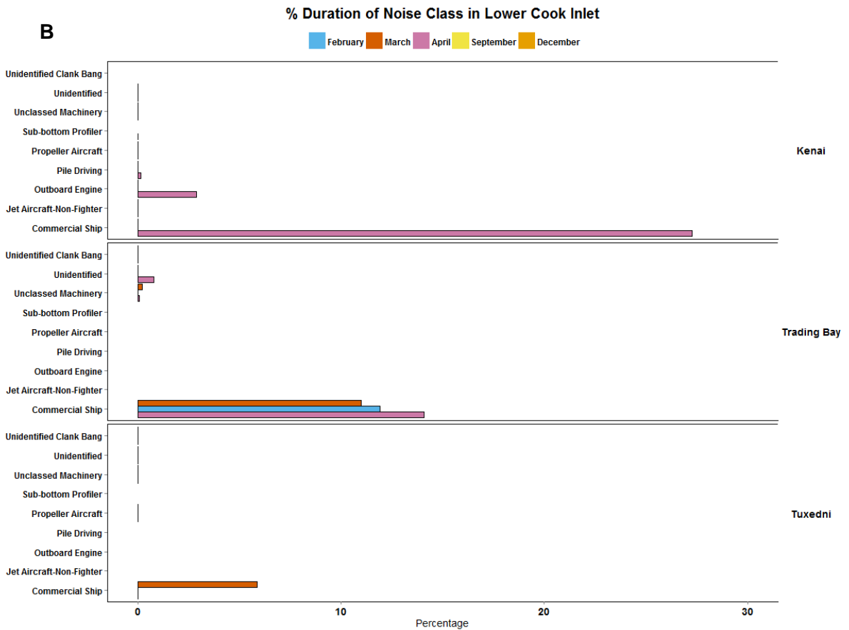
Figure 3: Percent duration of all the acoustic events detected at each site by month and noise class. Upper panel (A) includes the 4 locations sampled in the Upper Inlet (Cairn Point, Eagle River, Fire Island and Six Mile), and the lower panel (B) includes the 3 locations sampled in the Lower Inlet (Kenai, Trading Bay and Tuxedni). Percentages are calculated from the total amount of recording time for each month and location. Note that up to three months were selected per location (see table 1), therefore, not all months were sampled in all locations.
