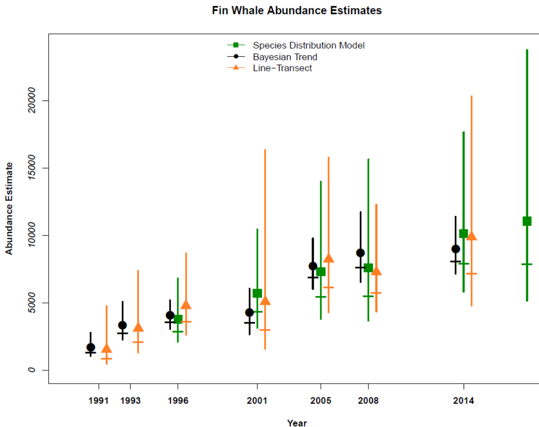
Figure 2. Fin whale abundance estimated from three methods (standard vessel-based line transect surveys (Barlow 2016), habitat-based species distribution models (Becker et al. 2020), and a Bayesian trend analysis (Nadeem et al. 2016). Vertical bars indicate approximate 95% log-normal confidence limits for line-transect estimates, 95% confidence limits reported from species distribution model estimates, and 95% prediction intervals from Nadeem et al. (2016). Line-transect surveys in 1991 and 1993 exclude Oregon and Washington waters. Horizontal hatch marks represent minimum population size estimates based on 20 th percentiles of mean estimates. Line-transect surveys in 1991 and 1993 did not include the waters of Oregon and Washington.
