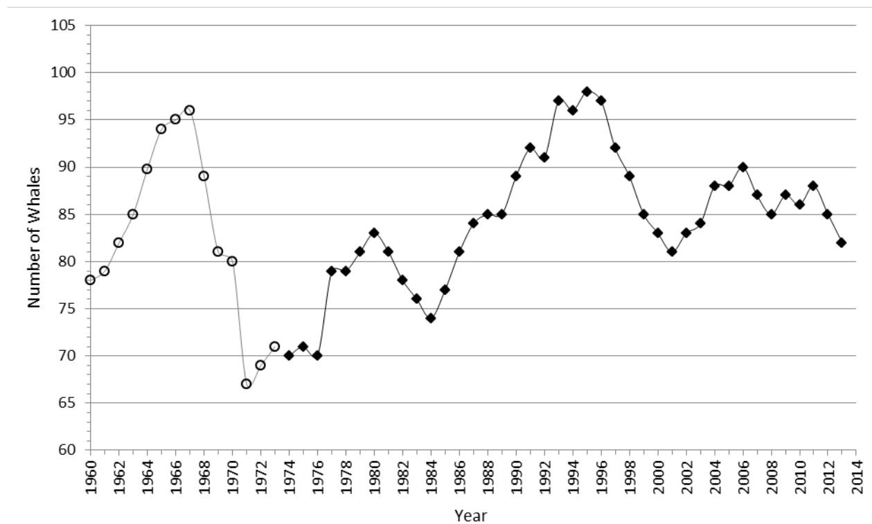
Figure 2.2-1. Population size and trend of Southern Resident killer whales, 1960-2013. Data from 1960-1973 (open circles, gray line) are number projections from the matrix model of Olesiuk et al. (1990). Data from 1974-2013 (diamonds, black line) were obtained through photo-identification surveys of the three pods (J, K, and L) in this community and were provided by the Center for Whale Research (unpublished data) and NMFS (2008). Data for these years represent the number of whales present at the end of each calendar year, except for 2013, when data only extend to July.
